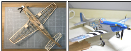
P-51D Mustang, 1:30, Clark-Y
